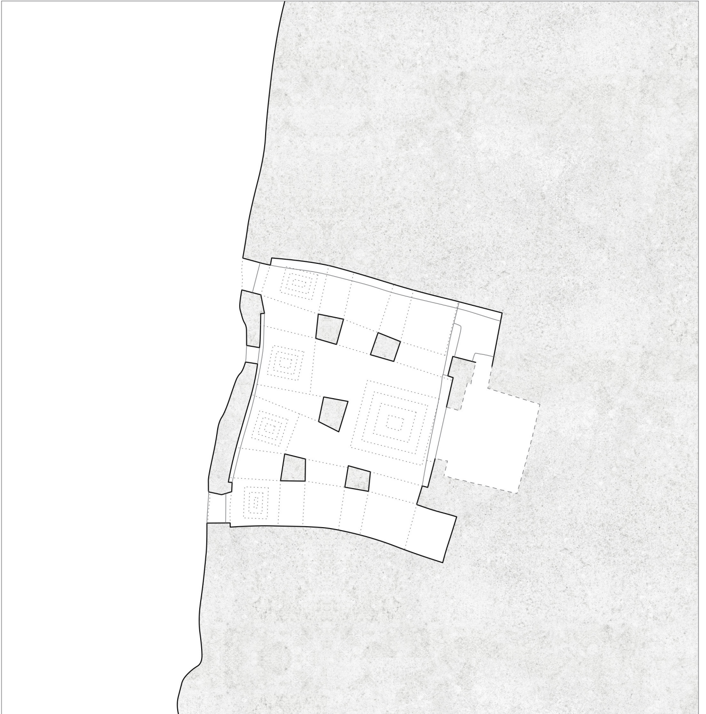
Giyorgis Manacheka Ground Floor Plan (2017)
